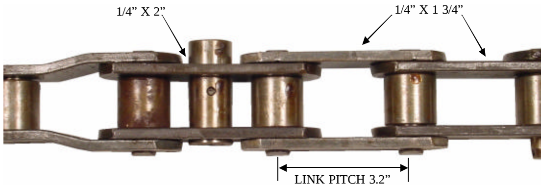
“N” STANDARD STEP CHAIN
